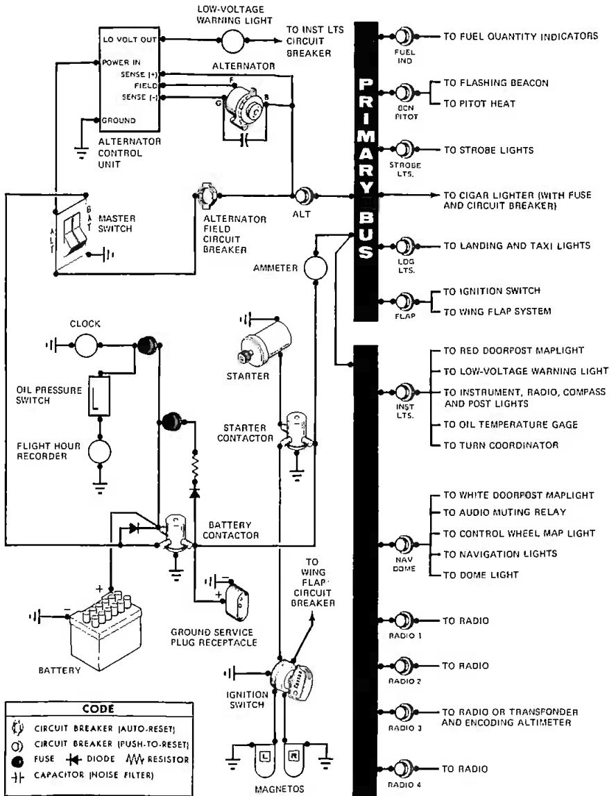
Figure 7-7. Electrical System
