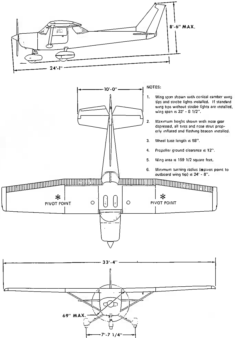
Figure 1-1. Three View
